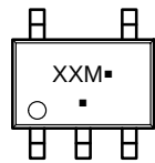
SC70-5 CASE 419AC
